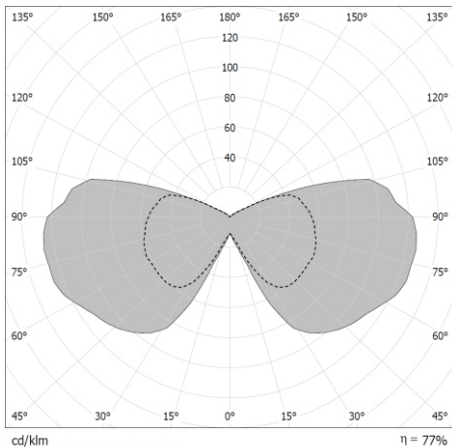
cd/klm C0 - C180 ..... C90 - C270 Photometry (polar plot) η = 77%
